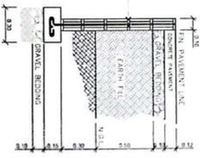
DETAIL OF WALL FOOTING SCALE 1 : 20M
