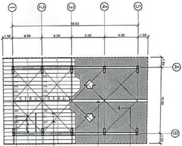
ROOF / ROOF FRAMING PLAN SCALE 1 : 200M
