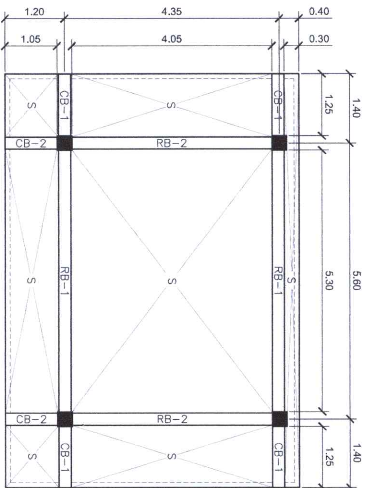
ROOF BEAM PLAN SCALE 1 : 75M
