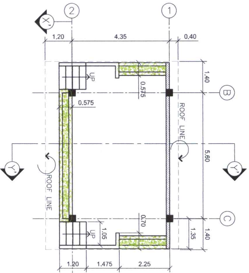
STAGE FLOOR PLAN SCALE 1 : 100M
