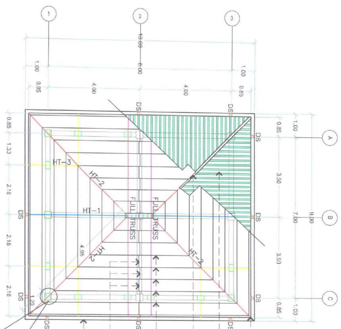
ROOF FRAMING PLAN SCALE 1 : 100M
