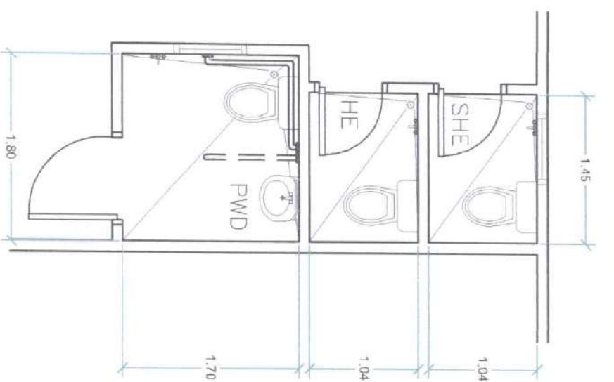
CR BLOW-UP DETAILS SCALE 1 : 50M
