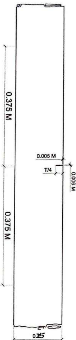
WEAKENED PLANE JOINT OR CONTRACTION JOINT SECTION B-B
