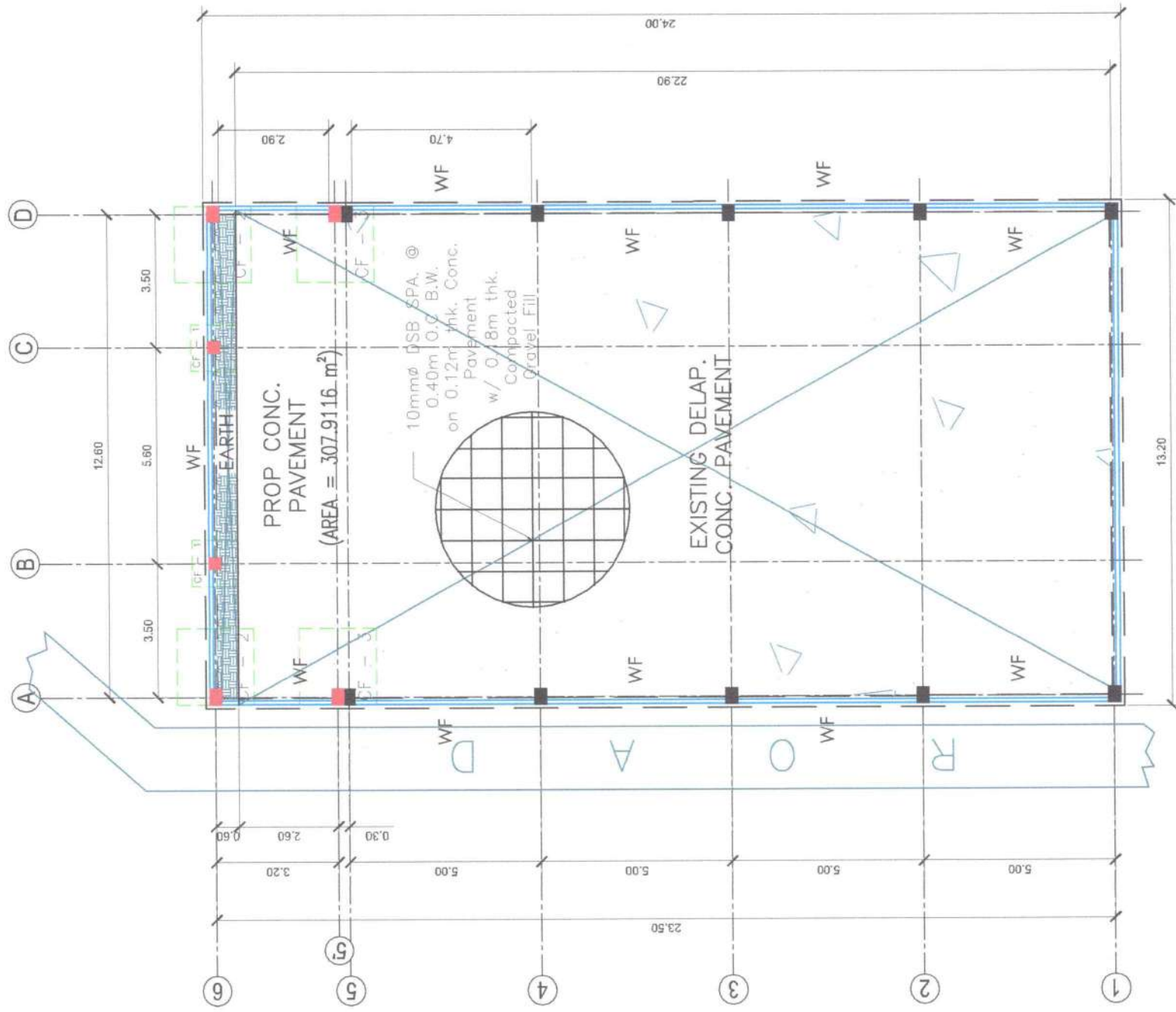
FLOOR PLAN / FOUNDATION PLAN SCALE 1 : 150M
