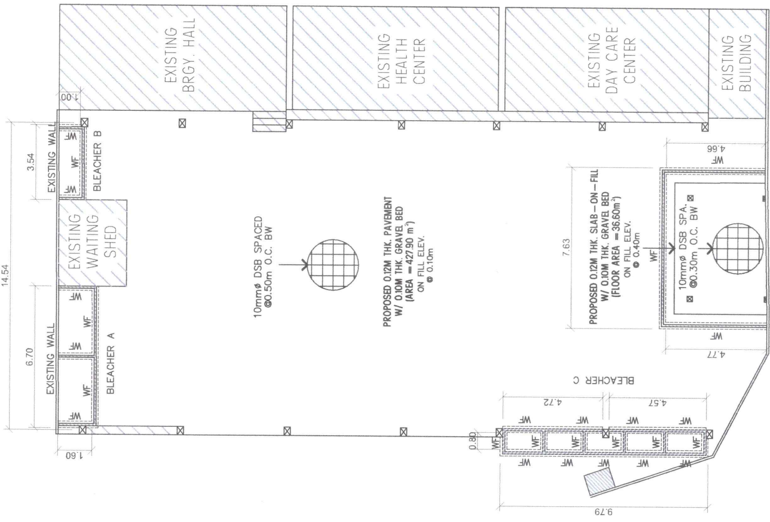
FOUNDATION PLAN SCALE: 1:175MTS
