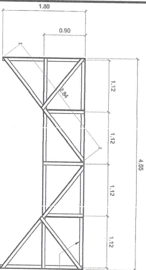
DETAIL ELEVATION STEEL STRUT-5 SCALE 1:50M
