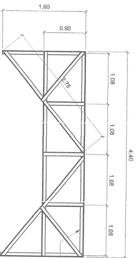
DETAIL ELEVATION STEEL STRUT-4 SCALE 1:50M
