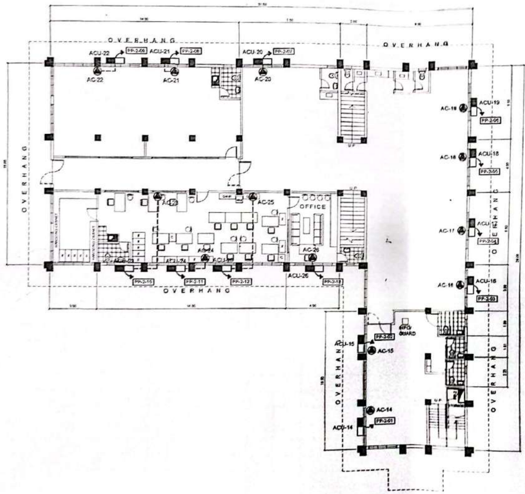
AIRCONDITIONING LAYOUT - SECOND FLOOR SCALE 1 : 200 M
