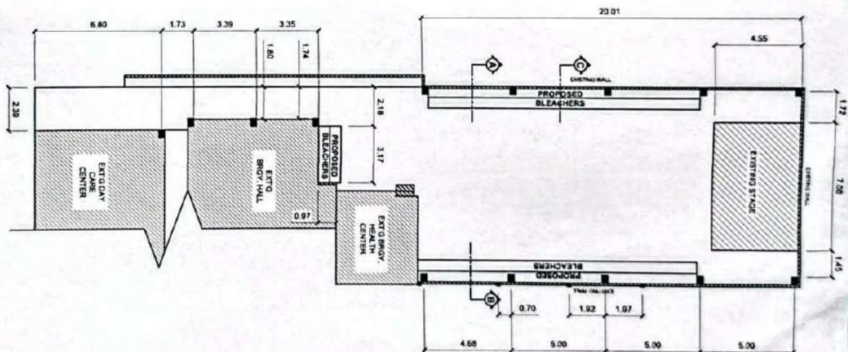
FLOOR PLAN SCALE 1:200M
