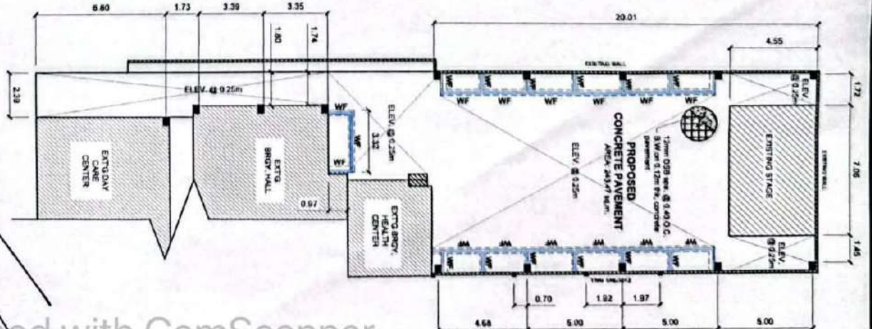
FOUNDATION PLAN SCALE 1:200M
