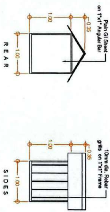
PLAN & ELEVATION OF PUMPHOUSE Scale 1:50
