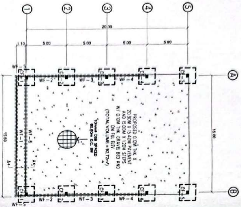
FOUNDATION PLAN SCALE 1 : 200M
