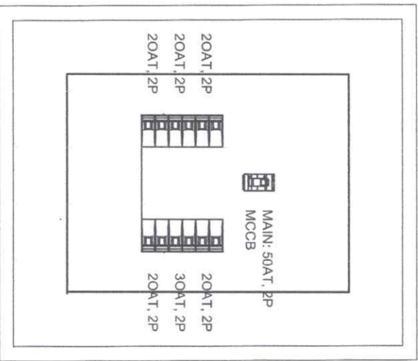
G.E. PANELBOARD 6 BRANCHES FLUSH MOUNTED
