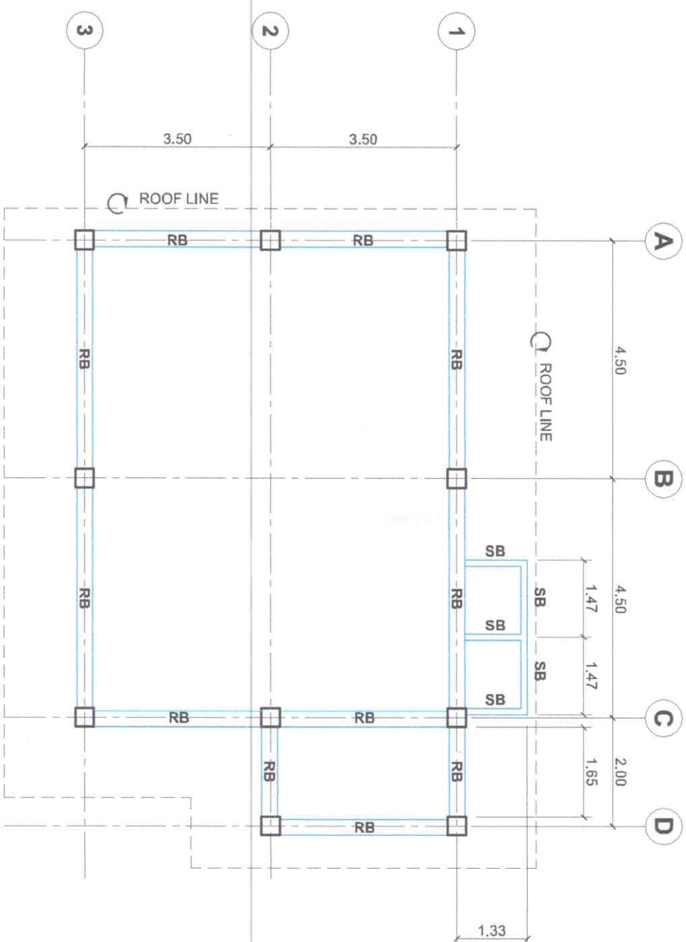
BEAM PLAN SCALE 1:100 MTS
