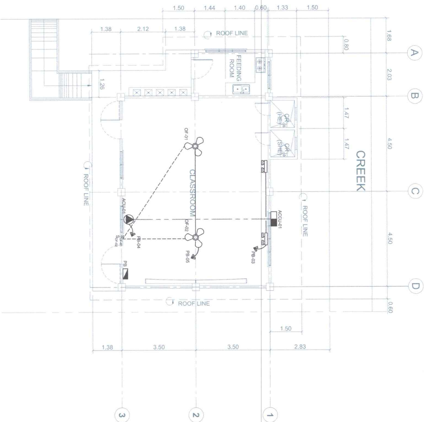
GROUND FLOOR – ACU & EMERG LIGHTING LAYOUT SCALE 1 : 100M
