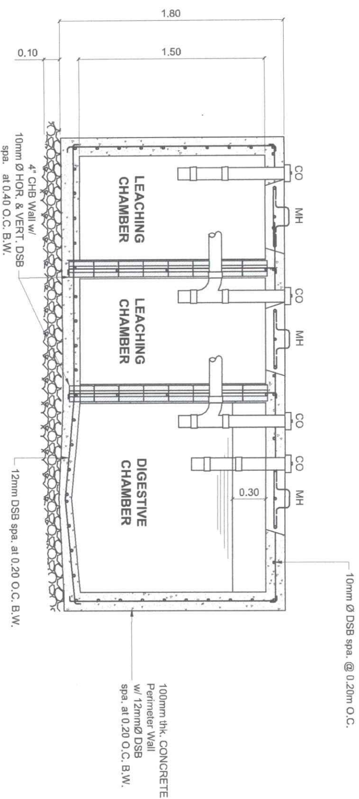
SECTION/ELEVATION
