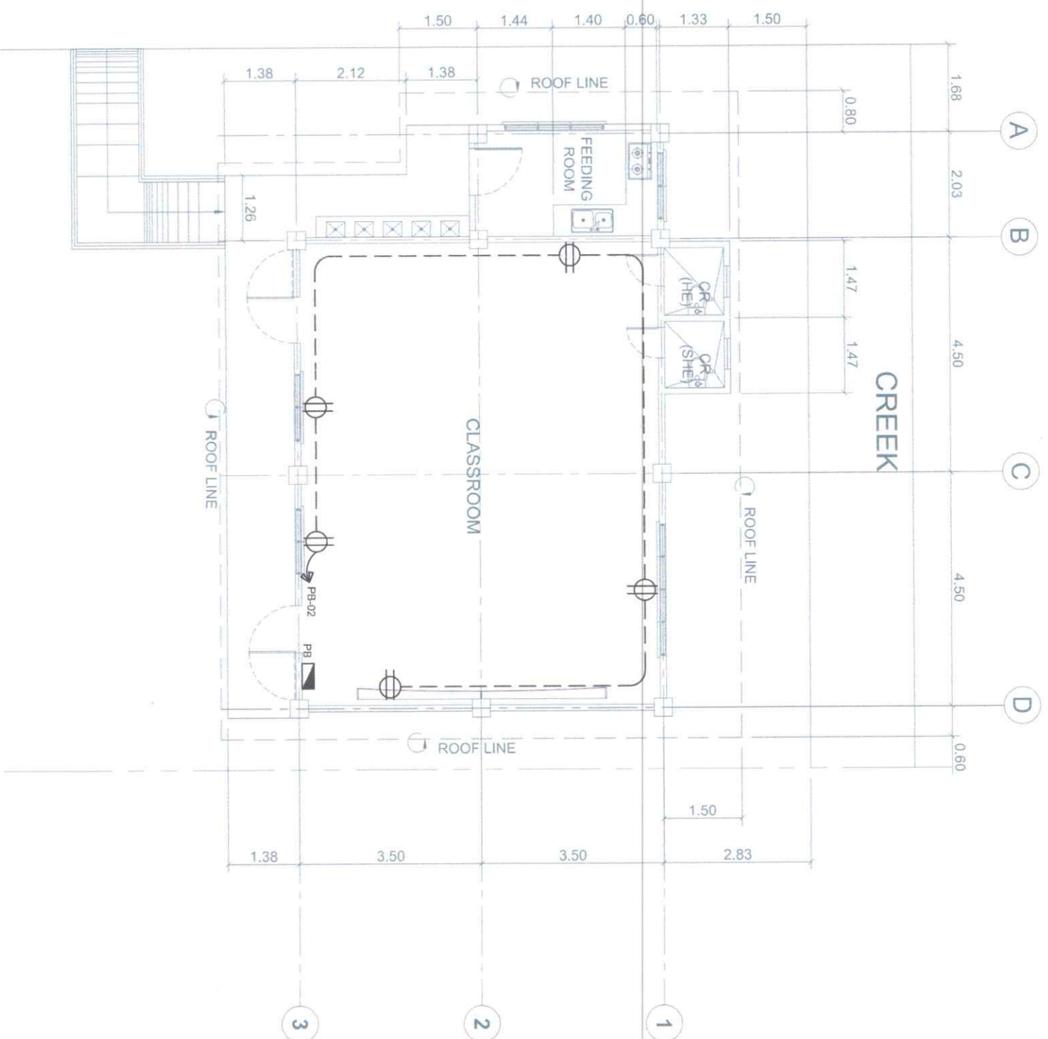
GROUND FLOOR – POWER LAYOUT SCALE 1 : 100M
