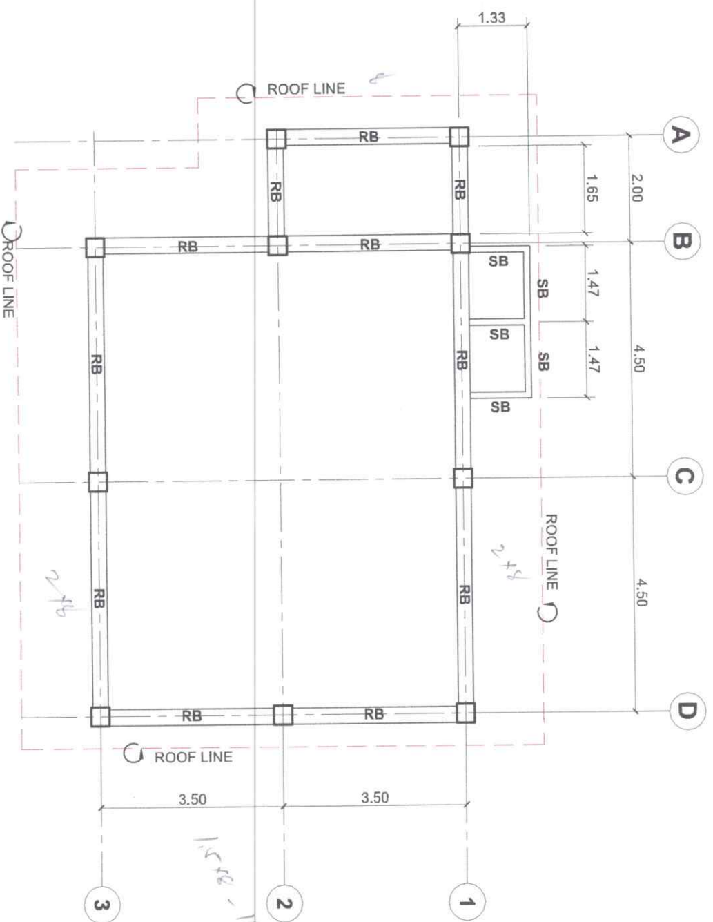
BEAM PLAN SCALE 1:100 MTS
